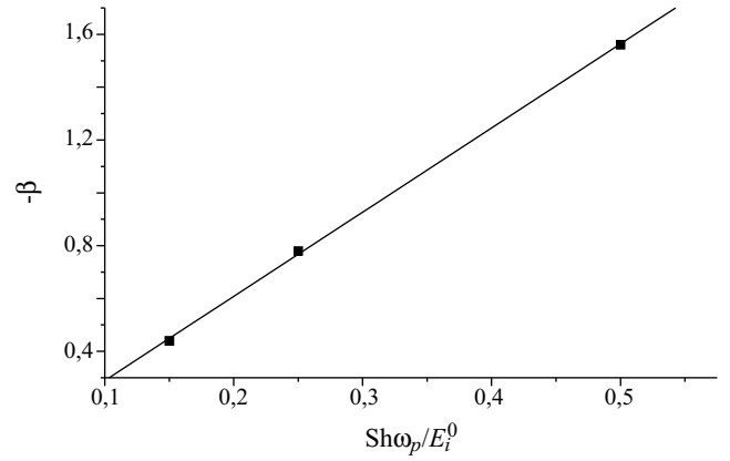
Figure 5 - Temperature coefficient of the apparent shift of energy with temperature ( \beta_T ) as a function of \frac{S\hbar\omega_p}{E_I^0} .
