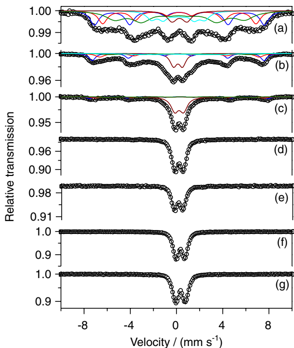
Figure 3. Room temperature Mössbauer spectra of (a) pure \text{Fe}_3\text{O}_4 (M0Z); composites of \text{Fe}_3\text{O}_4 and (b) 100 mg (M100Z); (c) 150 mg (M180Z); (d) 200 mg (M200Z); (e) 250 mg (M250Z); (f) 500 mg (M500Z) and (g) 1000 mg (M1000Z) of zeolite 13x.
