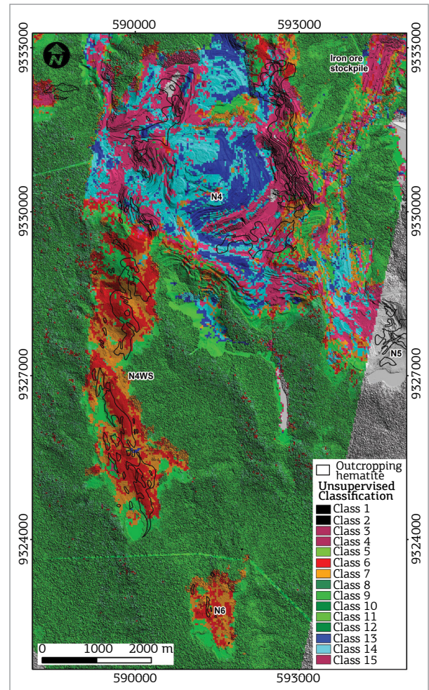
Figure 16. Class image resulting from unsupervised classification applied on Hyperion, gamma ray spectrometric data, Tzz gravimetric gradient component, and Landsat-8/OLI-derived Normalized Difference Vegetation Index data. The base image is a Laser Imaging Detection and Ranging digital terrain model artificially illuminated from northeast.
