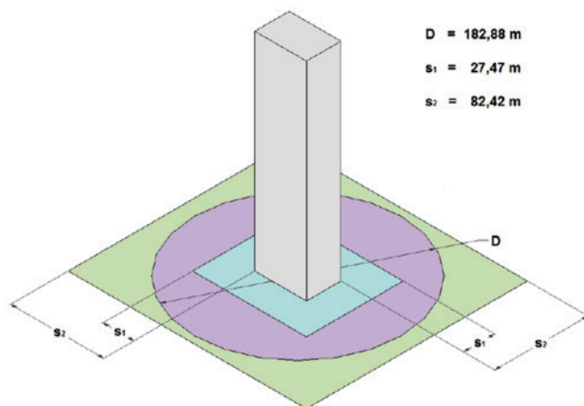
Figure 7 Union of the distance proposals of the strain standards on the CAARC standard building, according to the Brazilian standard
