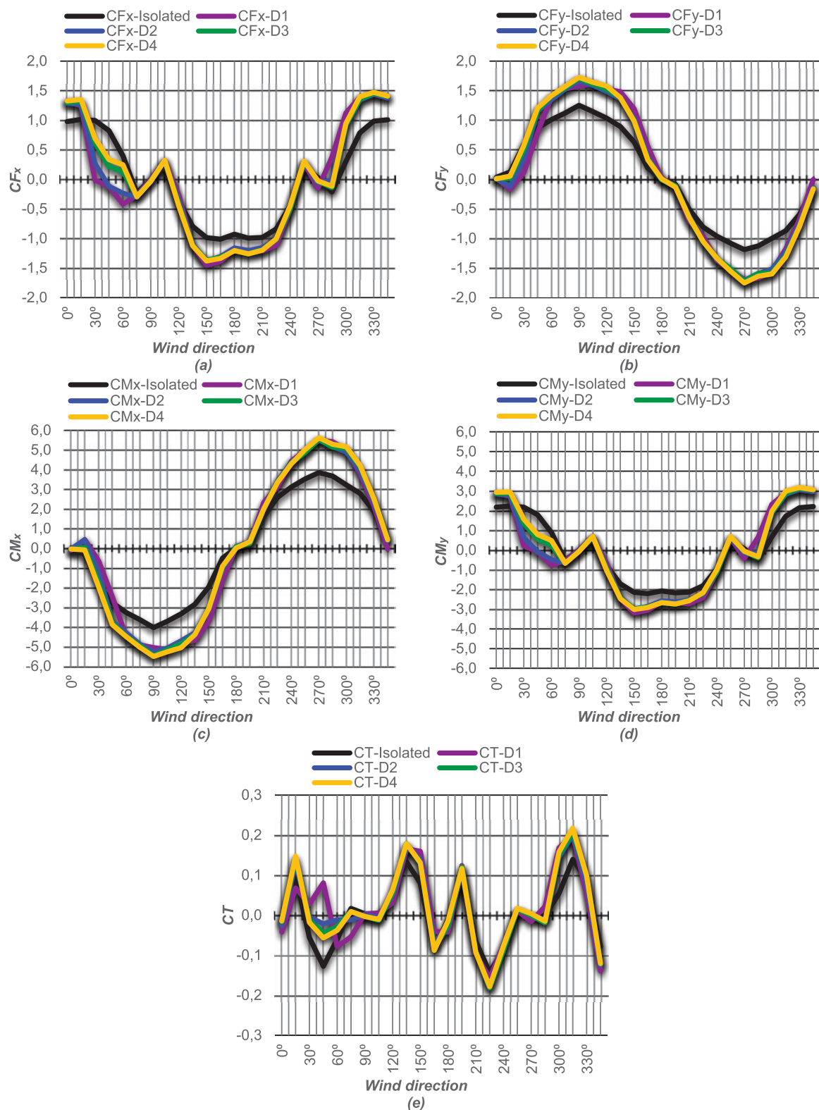
Figure 9 Load coefficients for the vicinity V2: (a) Resultant force in the direction of the X axis; (b) Resultant force in the direction of the Y axis; (c) Base momenta round axis X; (d) Base moment around axis Y; (e) Torsion around building axis
