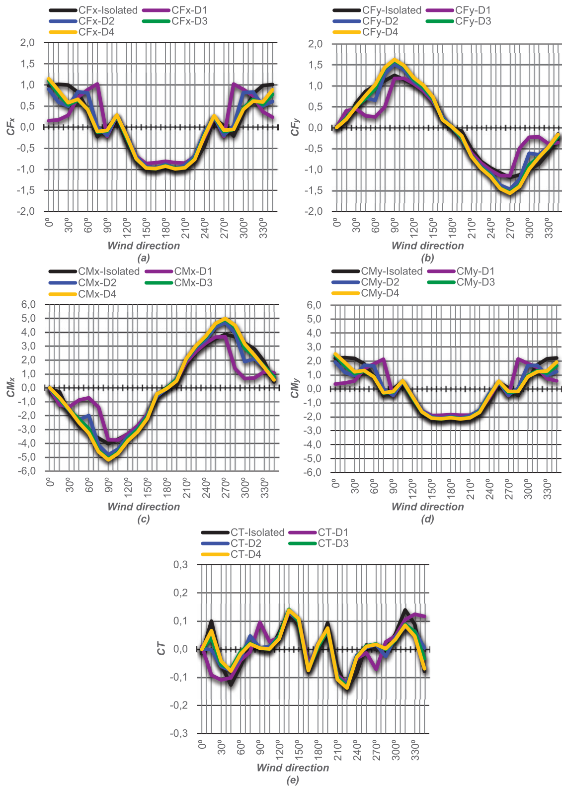
Figure 15 Load coefficients for the vicinity V8: (a) Resultant force in the direction of the X axis; (b) Resultant force in the direction of the Y axis; (c) Base momenta round axis X; (d) Base moment around axis Y; (e) Torsion around building axis
