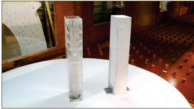
Figure 2 Instrumented model and CAARC standard building muted model
