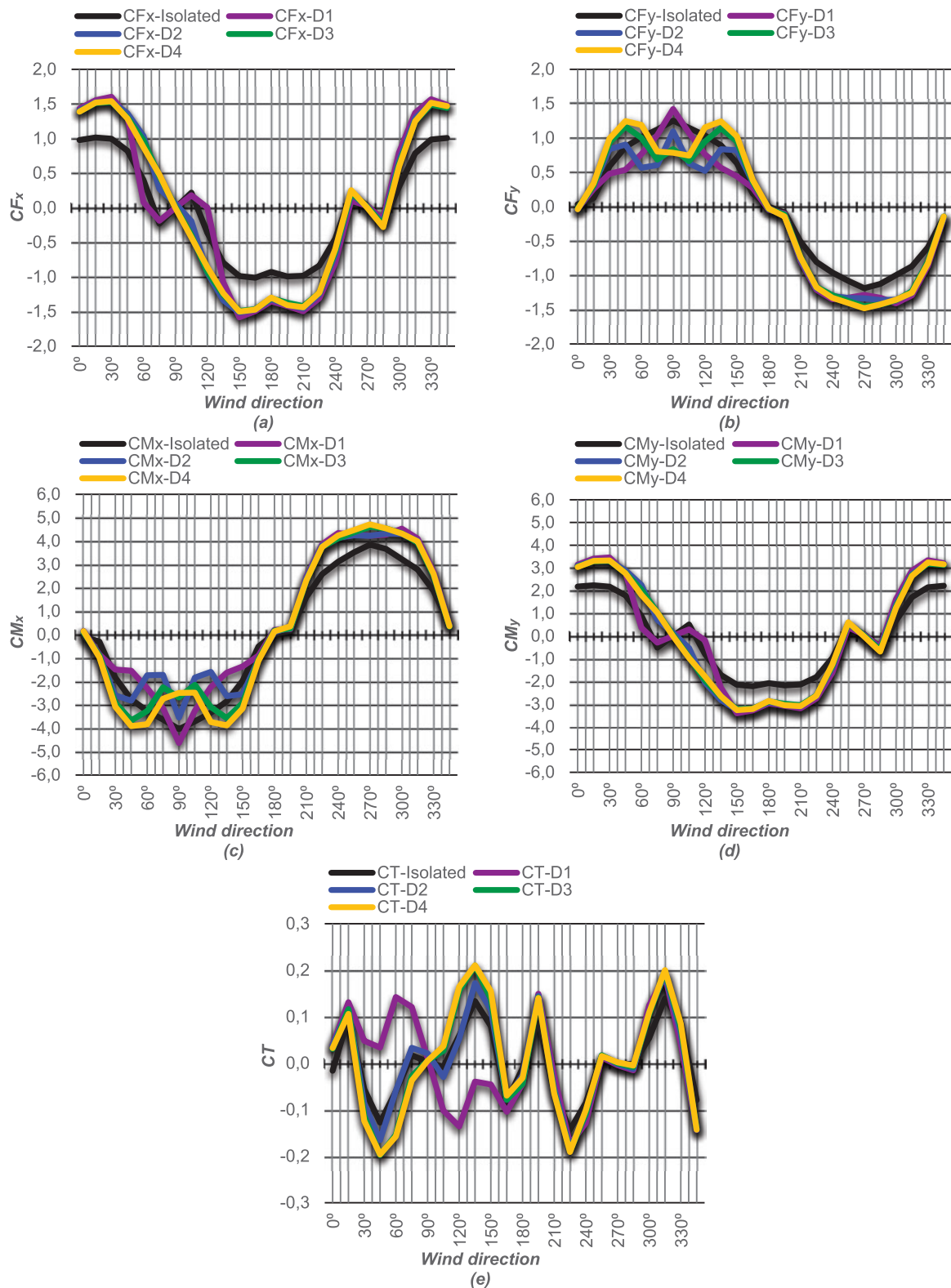
Figure 11 Load coefficients for the vicinity V4: (a) Resultant force in the direction of the X axis; (b) Resultant force in the direction of the Y axis; (c) Base momenta round axis X; (d) Base moment around axis Y; (e) Torsion around building axis
