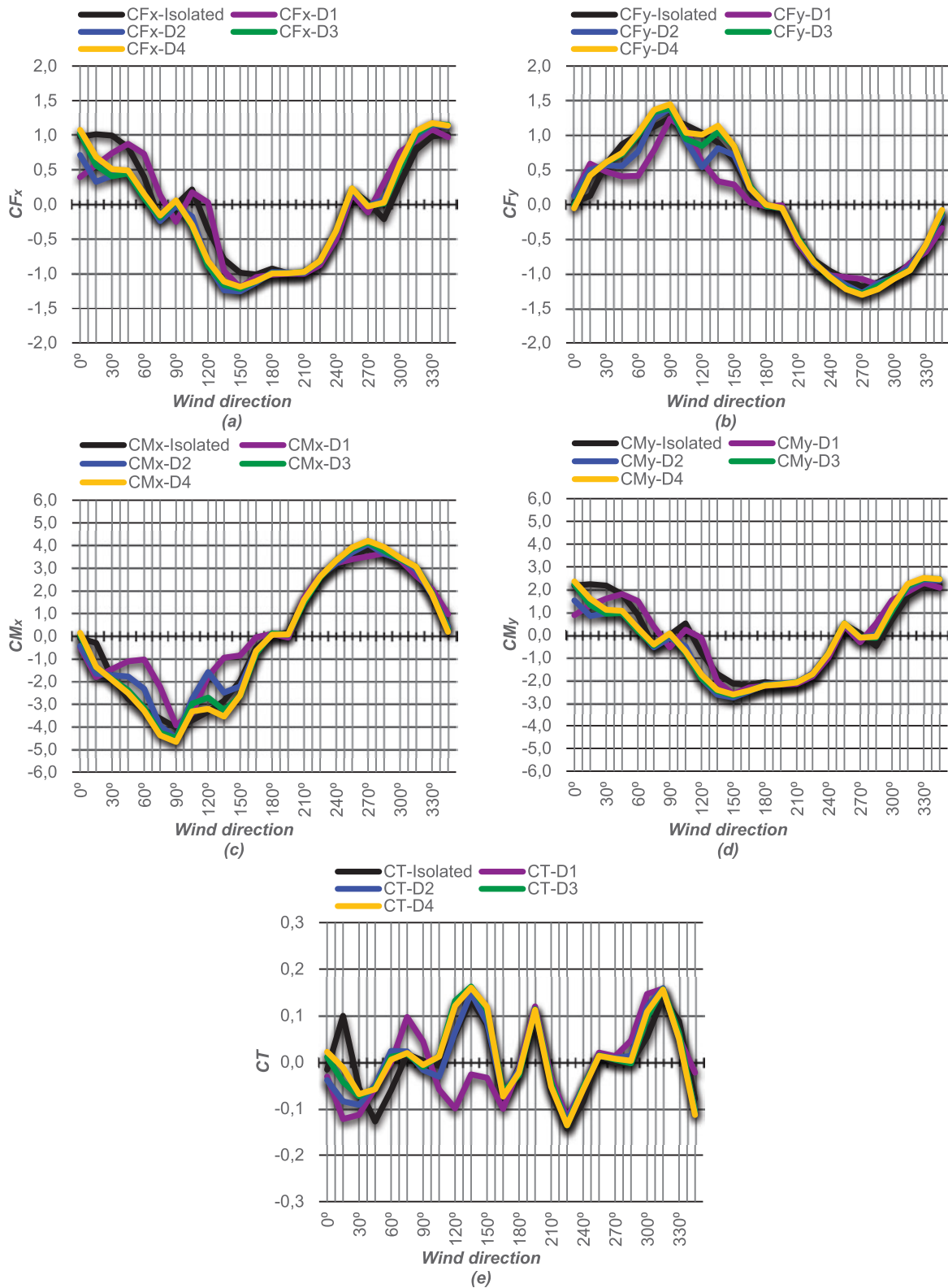
Figure 13 Load coefficients for the vicinity V6: (a) Resultant force in the direction of the X axis; (b) Resultant force in the direction of the Y axis; (c) Base momenta round axis X; (d) Base moment around axis Y; (e) Torsion around building axis
