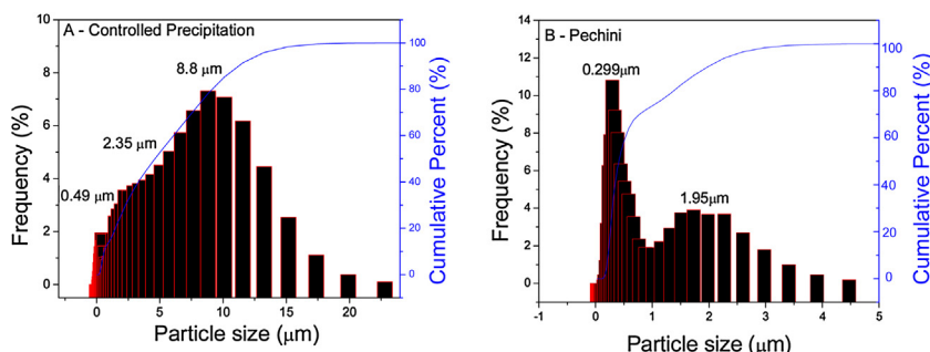
Fig. 1 – Particle size distribution of Ce 0.80 Gd 0.19 Sm 0.01 O 1.9 powders using the controlled precipitation (A) and Pechini (B) methods.
