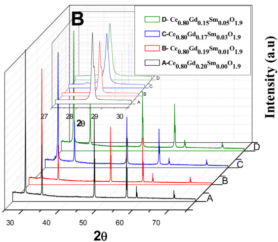
Fig. 8 – X-ray diffractograms of electrolytes sintered from powders synthesized by the controlled precipitation (A) and Pechini (B) methods.
