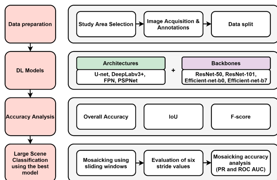
Figure 1. Methodological flowchart.
