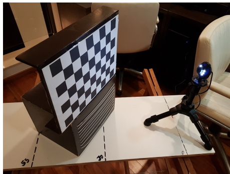
Figure 2.6: Calibration object used in the experiments.
