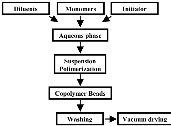
FIG. 1: Flowchart for preparation of copolymer micro-spheres.
