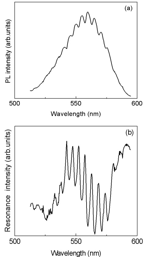
FIG. 3: (a) Low temperature (77 K) PL spectra of single polymer sphere. (b) Normalized photoluminescence spectrum shows whispering-gallery modes.
