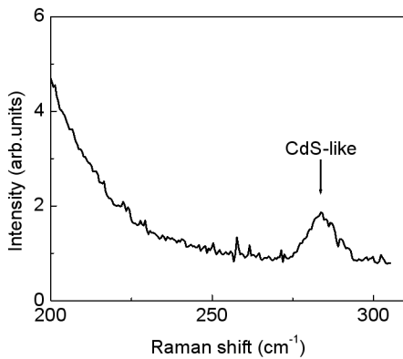
FIG. 2: Raman spectrum of CdS nanoparticles embedded in polymer microspheres measured at room temperature. The wavelength of excitation laser line is 488.0 nm.
